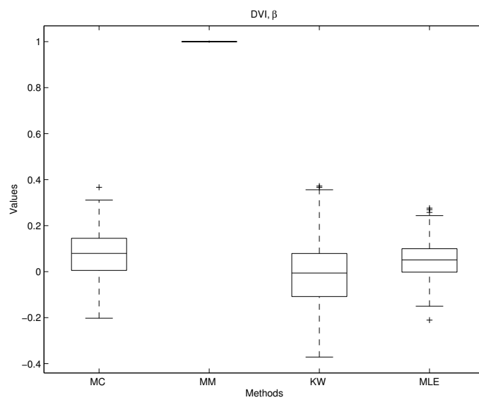
Figure 10: Boxplot diagrams of \hat{\beta} , DVI Inc.
