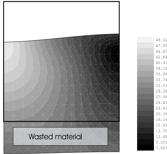
Figure 4: Amplified (by 60) deformed mesh and von Mises stress norm at final time T = 1 s and initial boundary.
