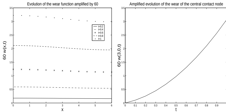
Figure 5: Wear of the contact boundary for several time values amplified by 60 and evolution of the wear of the central contact node.
