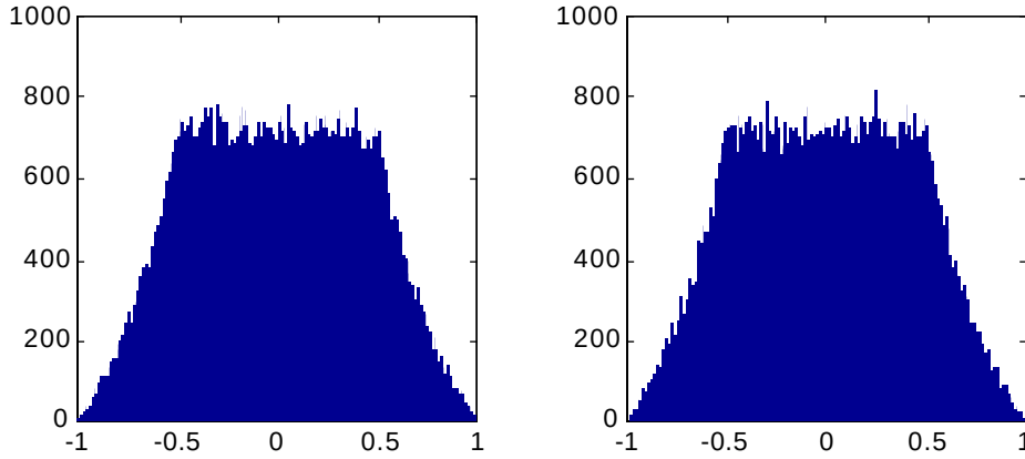
Figure 2: Distribution of roundoff errors \varepsilon^\times/u from multiplication of standard Gaussian data (left) and data distributed uniformly on [1, 2] (right), with 100000 samples.
