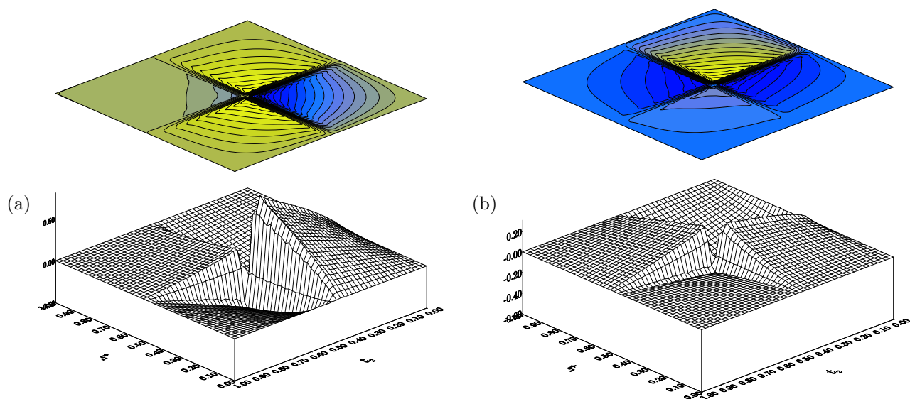
FIGURE 1. Surface and contour plots of the Peano type kernels P defined in (17) for different weights. (a) w(t_1, t_2) = -\ln(t_1 t_2) over the unit square and x_1 = x_2 = 0.5 , (b) w(t_1, t_2) = \sqrt{t_1/t_2} over the unit square and x_1 = x_2 = 0.5 .
