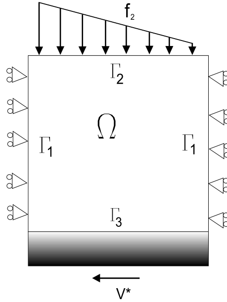
Figure 3: Test 2: Contact of a 2D viscoelastic body.
