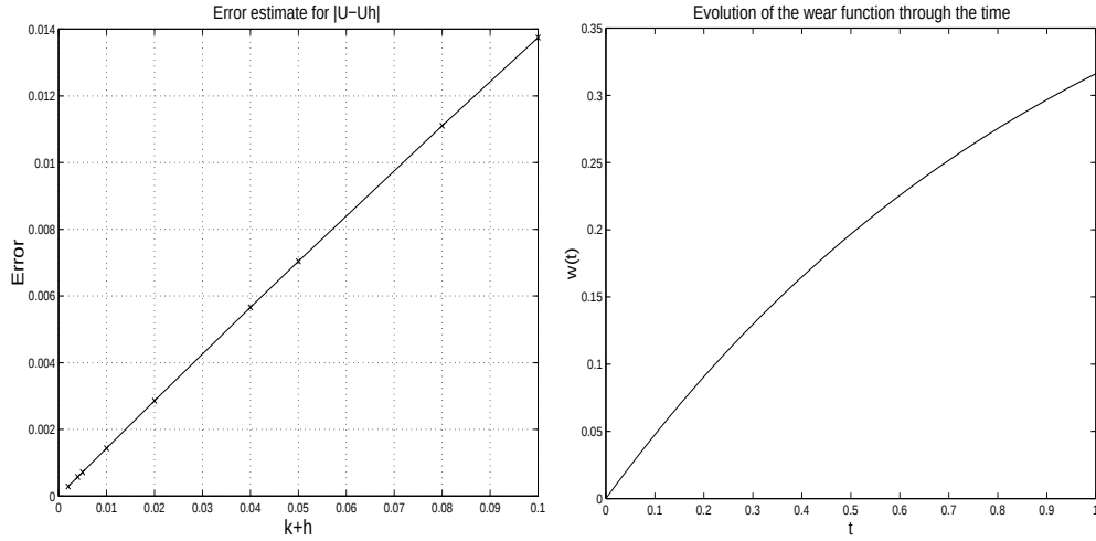
Figure 2: Problem T1D : Asymptotic constant of error and evolution of the wear function through the time.
