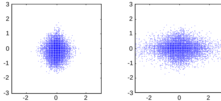
Figure 3: Distribution of roundoff errors \varepsilon^\times/u for different methods of complex multiplication
