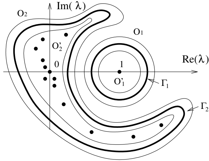
Figure 1: Spectrum of T(z_0) .
