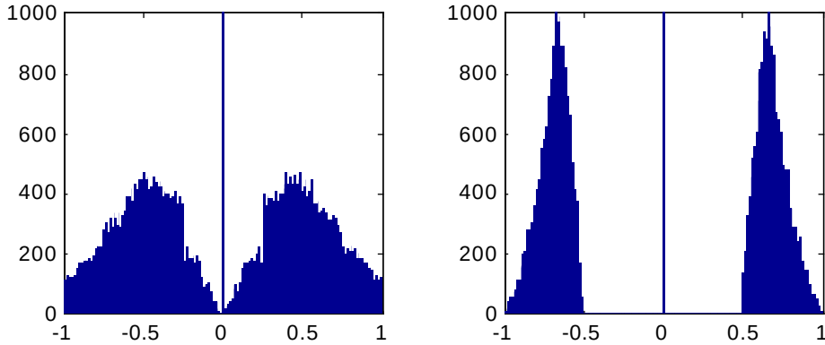
Figure 1: Distribution of roundoff errors \varepsilon^+/u from summation of standard Gaussian data (left) and data distributed uniformly on [1, 2] (right), with 100000 samples.
