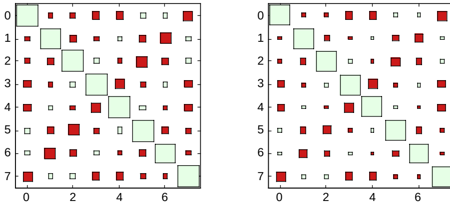
Figure 4: Computed (right) and simulated (left) covariance matrix for the roundoff errors of the fast DCT-II, followed by the fast DCT-III. The areas are proportional to the absolute values of the covariance and negative covariances are depicted by a darker shading.
