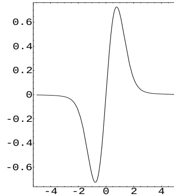
Figure 2: \psi_+^0(x)
