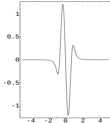
Figure 1: \psi_+^{2;(2,2)}(x)
